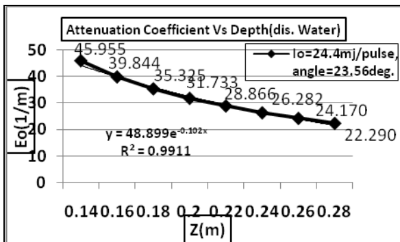
FIGURE 3. Less attenuation coefficients due to bigger angle in different depths (distilled water).
